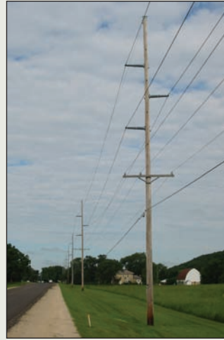
69-kV/115-kV transmission structure with distribution underbuild
